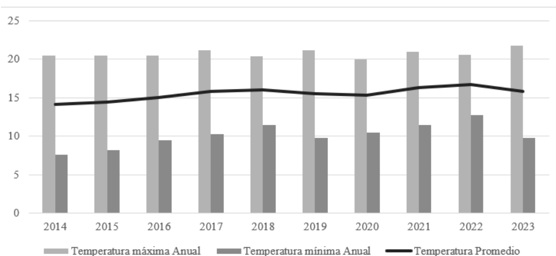
Figure 3. Maximum, average, and minimum temperatures in the village of San Antonio for the period 2014-2023
