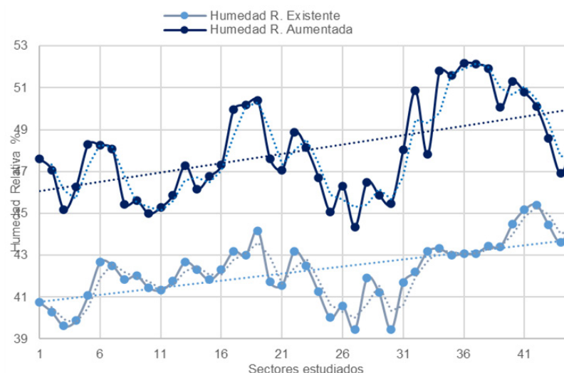
Figure 9. Relationship between relative humidity measured in the field and increase through passive mitigation strategies
