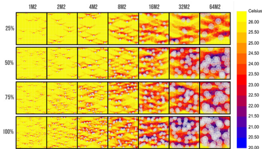
Figure 6. Plant material heights and vegetation cover effectiveness on shade projection vs. tree density
