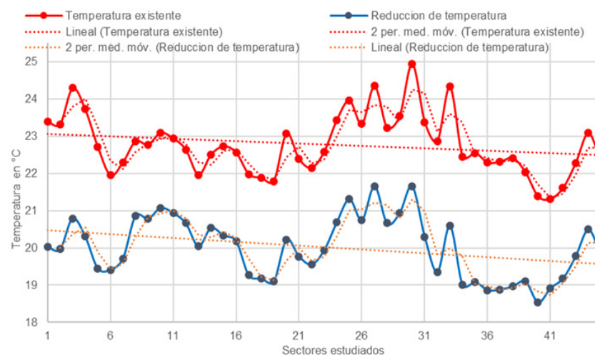
Figure 8. Relationship between temperature measured in the field and reduction through passive mitigation strategies
