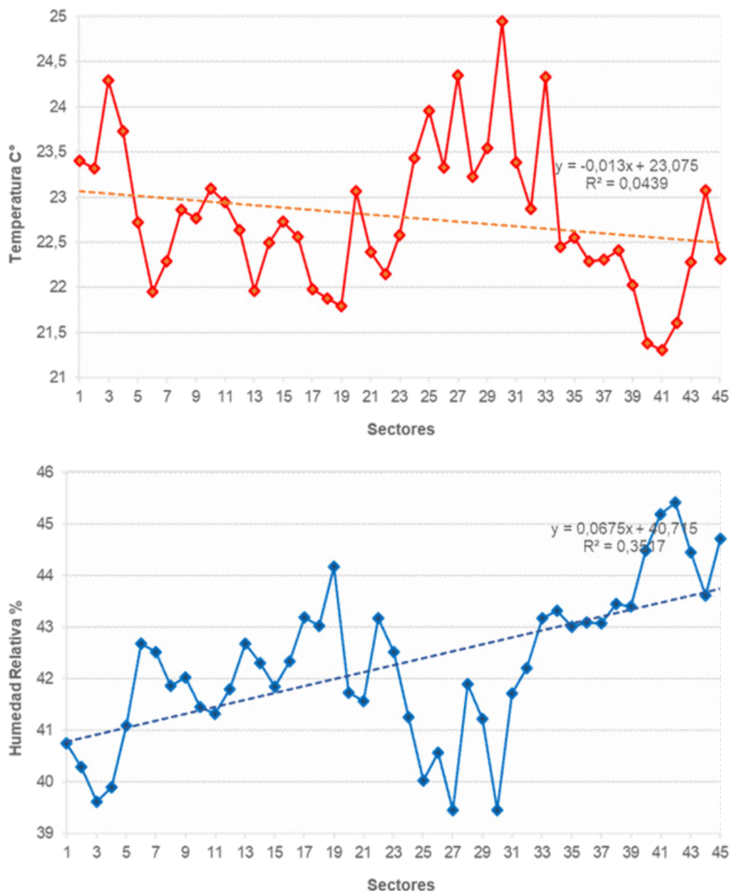
Figure 3. Ambient temperature and relative humidity data on the north-south connection, under measurement protocol
